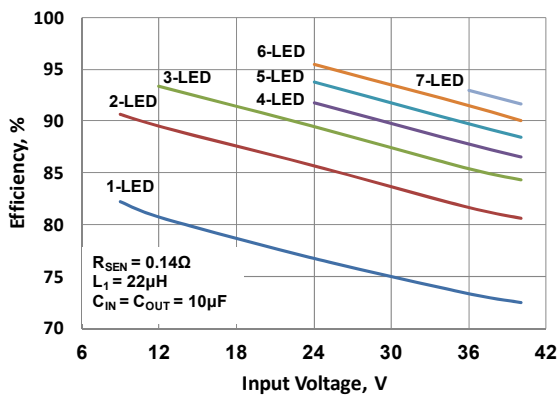
(a) L_1 = 22\mu H
